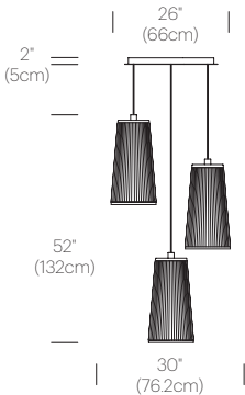
SOLIS CHANDELIER 3 (24")
