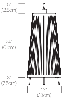
SOLIS FS 24
