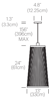
SOLIS 24
