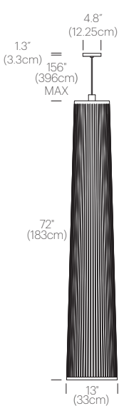
SOLIS 72
