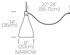
POWER FEED CABLE
